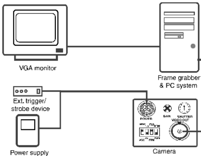
Figure 2. Camera and Frame Grabber System Setup
