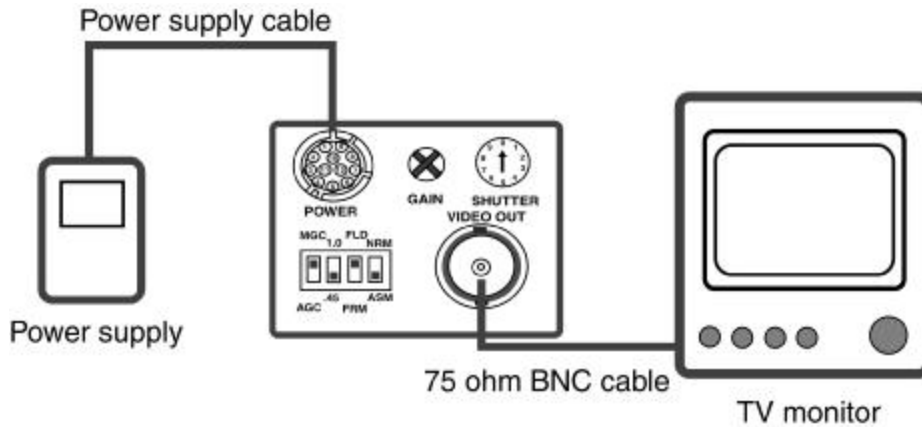
Figure 1. Basic Camera Setup
